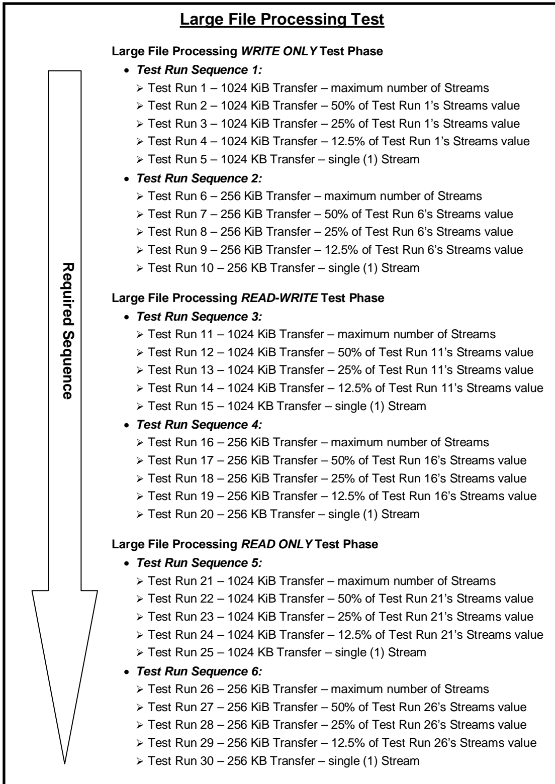
Figure 6-3: Summary of SPC-2 Tests
