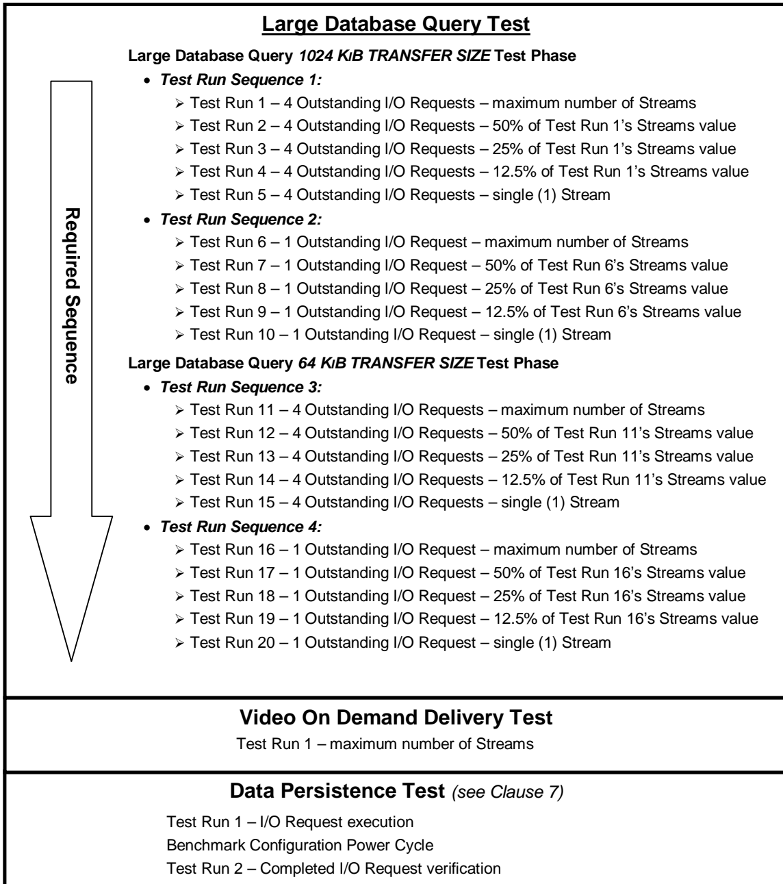
Figure 6-4: Summary of SPC-2 Tests (continued)
