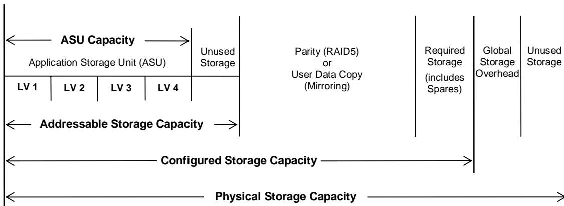
Figure 10-12: SPC-2 Storage Capacities and Relationships
