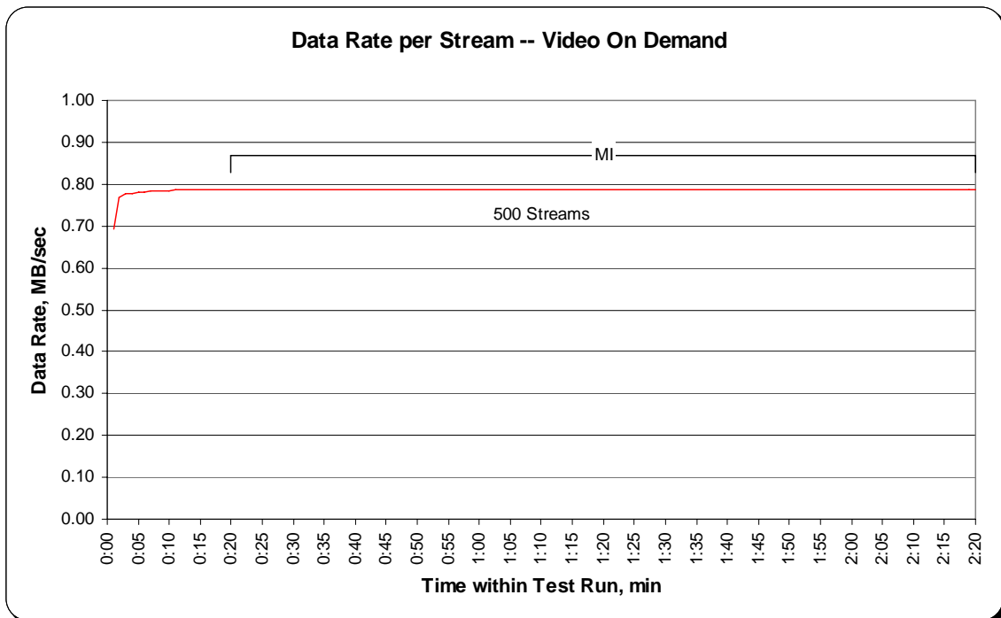
Figure 10-8: Average Data Rate per Stream by Intervals Graph (VOD)
