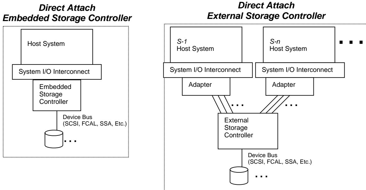
Figure 4-1: Benchmark Configuration – Direct Attach Storage Controller
