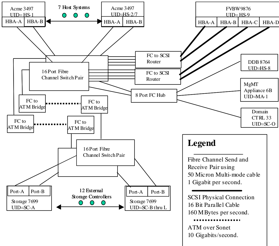
Figure 10-12: Storage Network Configuration Diagram
