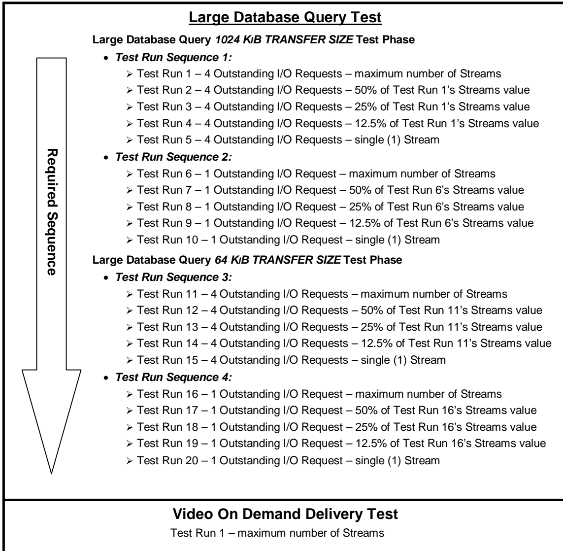
Figure 6-4: Summary of SPC-2 Tests (continued)
