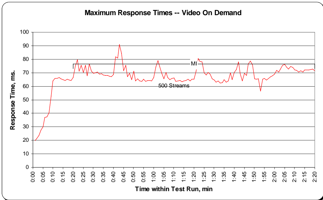
Figure 10-10: Maximum Response Time by Intervals Graph (VOD)
