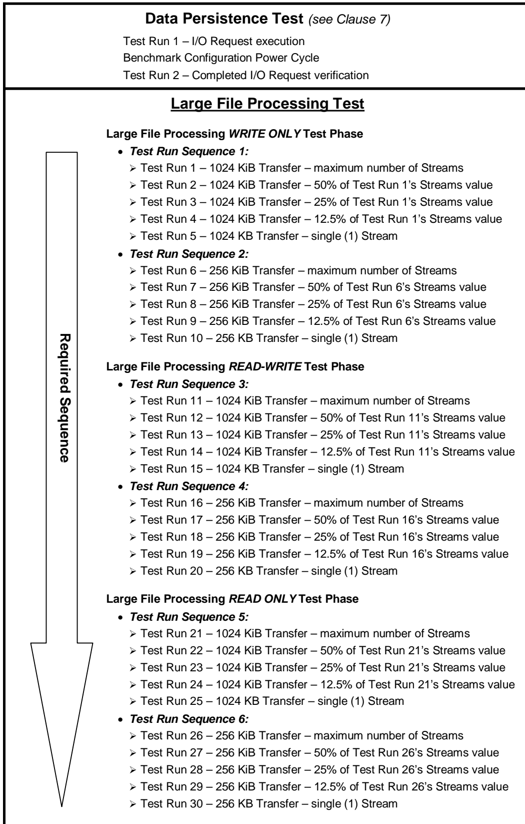
Figure 6-3: Summary of SPC-2 Tests
